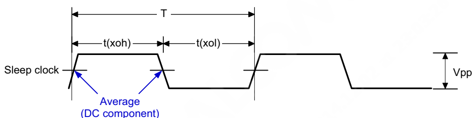
Figure 3-16 Sleep-clock timing parameters
