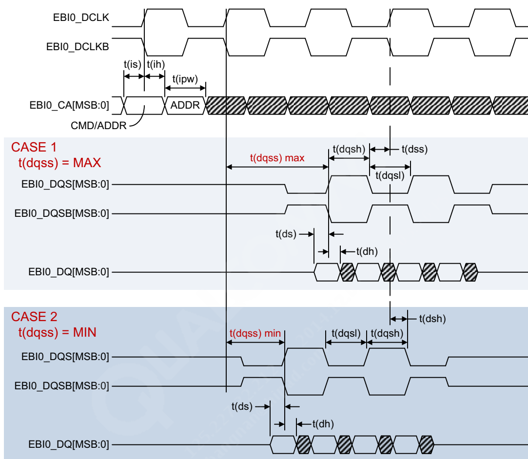
Figure 3-9 DDR SDRAM write timing
