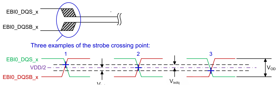
Figure 3-7 DDR SDRAM DQS_x and DQSB_x
