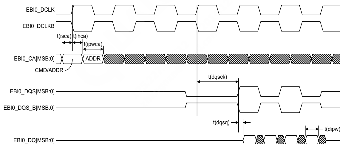
Figure 3-10 DDR SDRAM read timing
