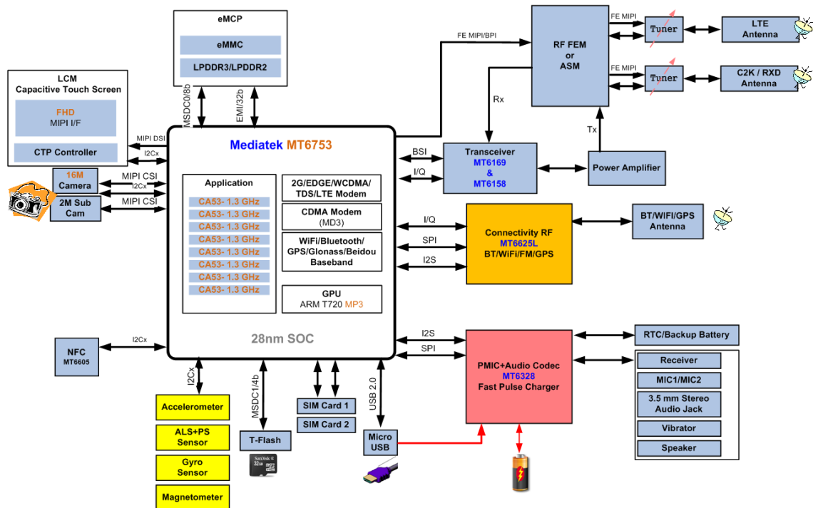
Figure 1-1. High-level MT6753 functional block diagram
