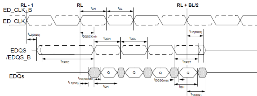
Data output (read) timing ( t_{DQCKmin} )
