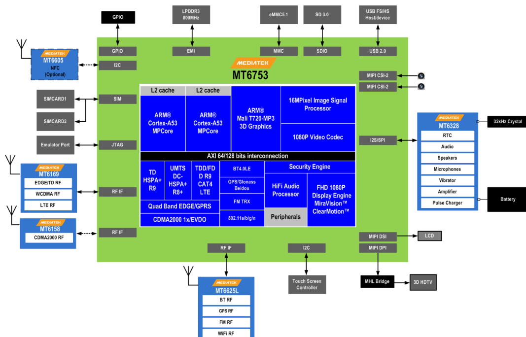
Figure 1-2. Block diagram of MT6753
