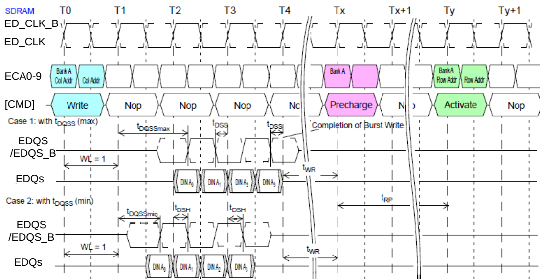
Figure 2-7. Basic timing parameter for LPDDR2 commands
