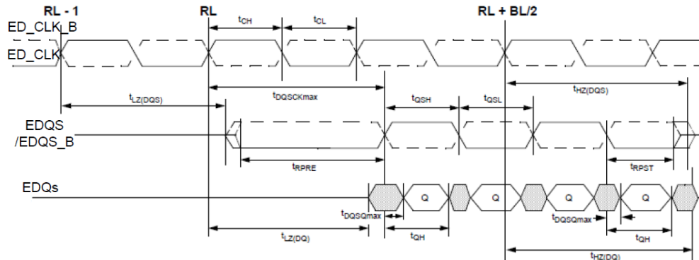
Data output (read) timing ( t_{DQCKmax} )
