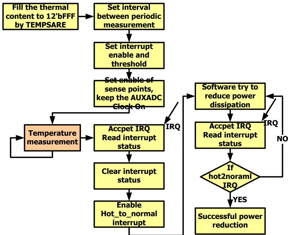
Figure 5-30. Programming flow
