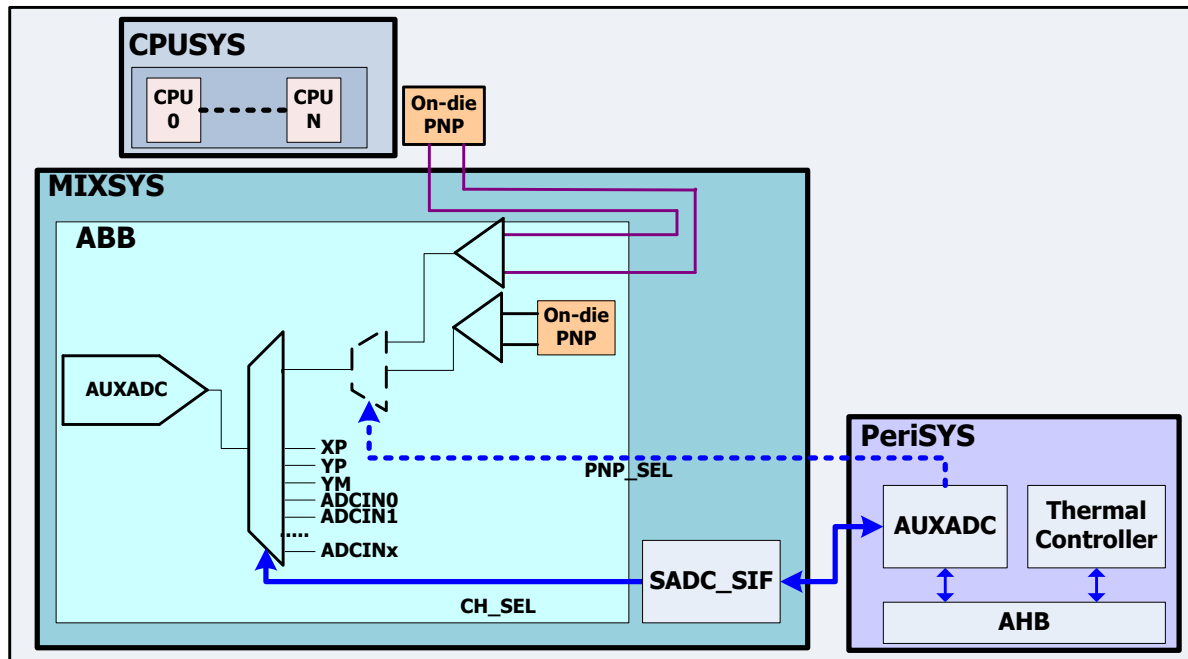
Figure 5-28. Block diagram of system temperature measurement
