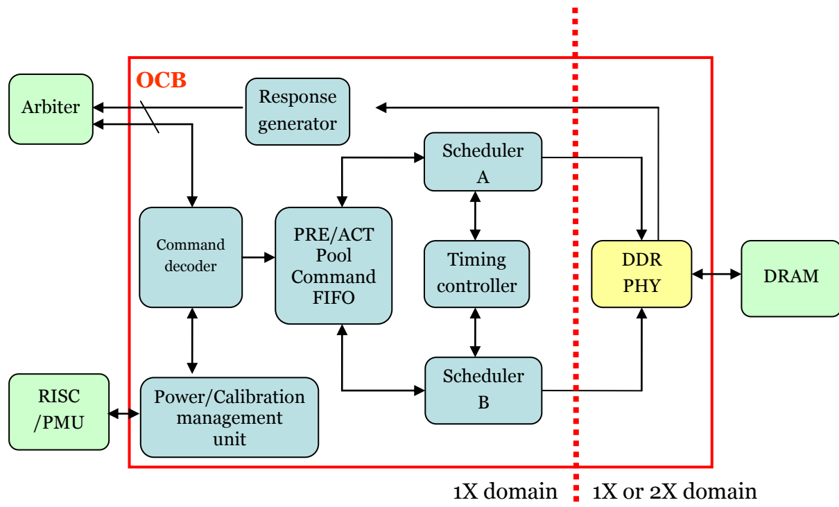
Figure 3-8. Block diagram of DRAM controller
