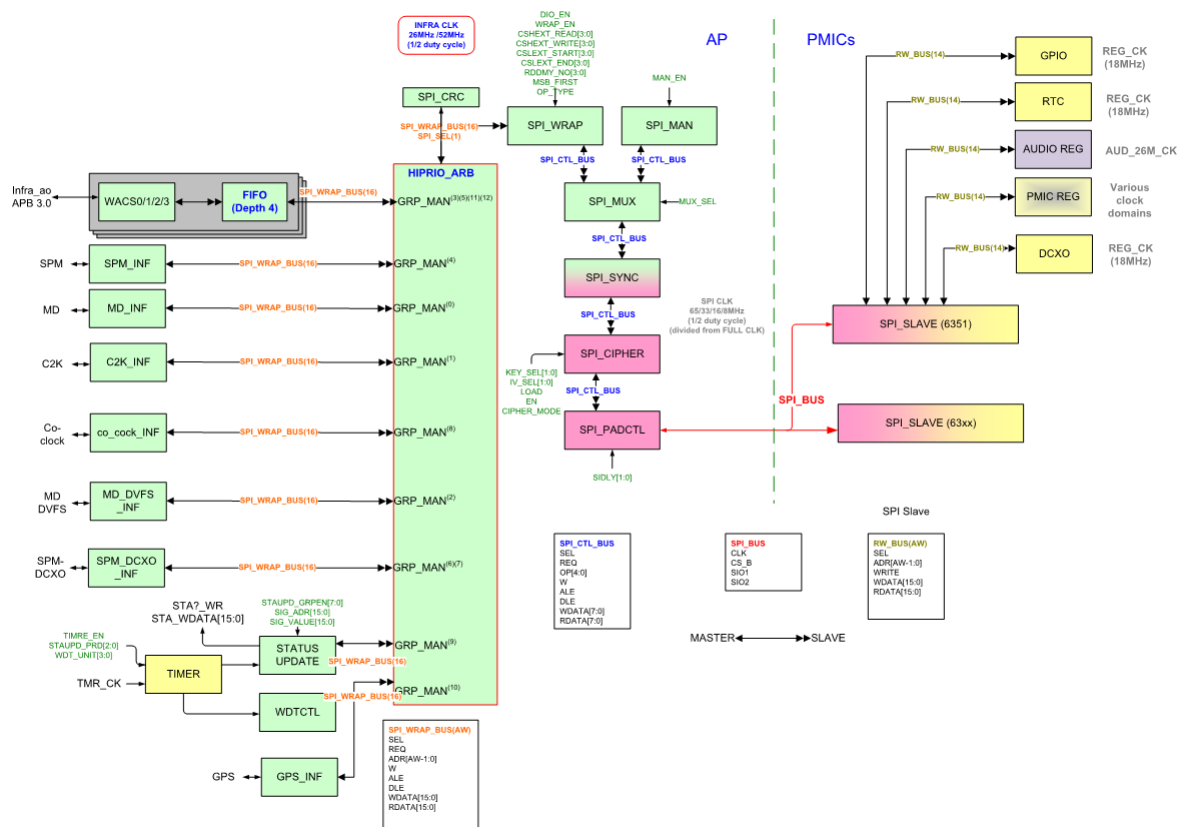
Figure 4-6. PMIC_WRAP architecture
