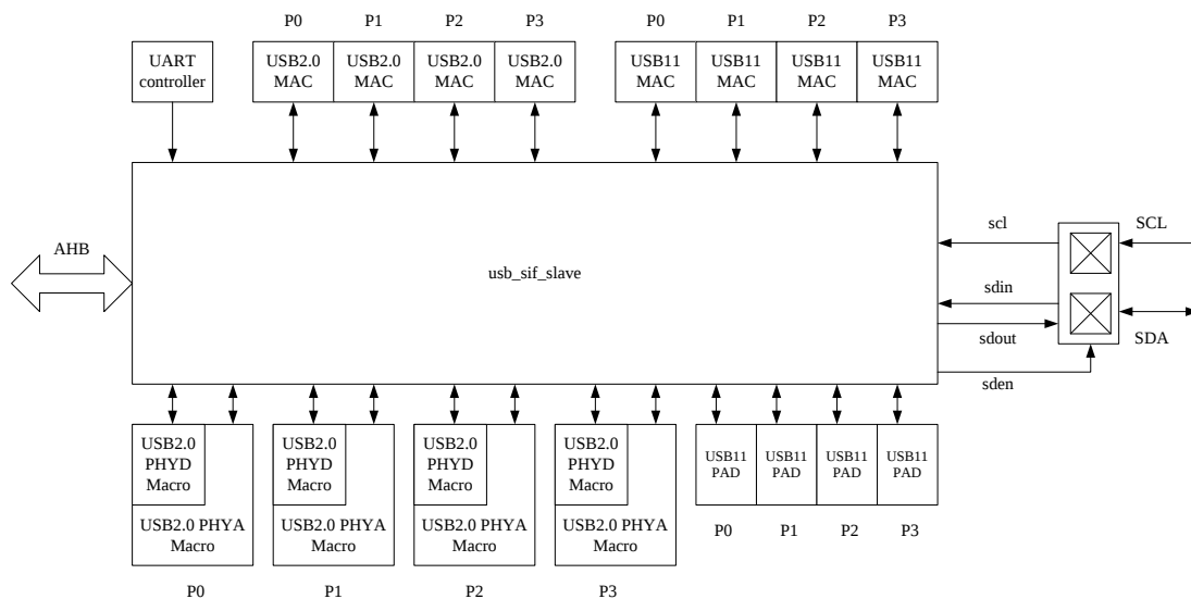
Figure 5-14. USBPHY RegFile block diagram
