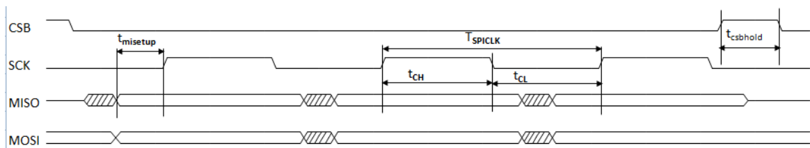
Figure 2-5. SPI timing diagram
