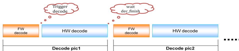
Figure 6-15. VDEC decoding flow
