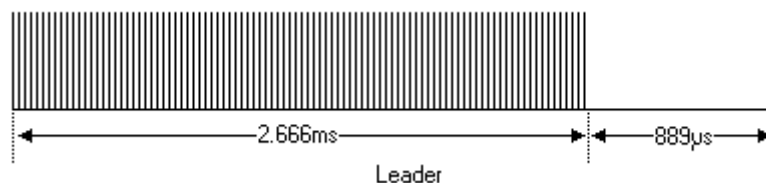
Figure 5-41. Lead pulse in RC6 protocol
