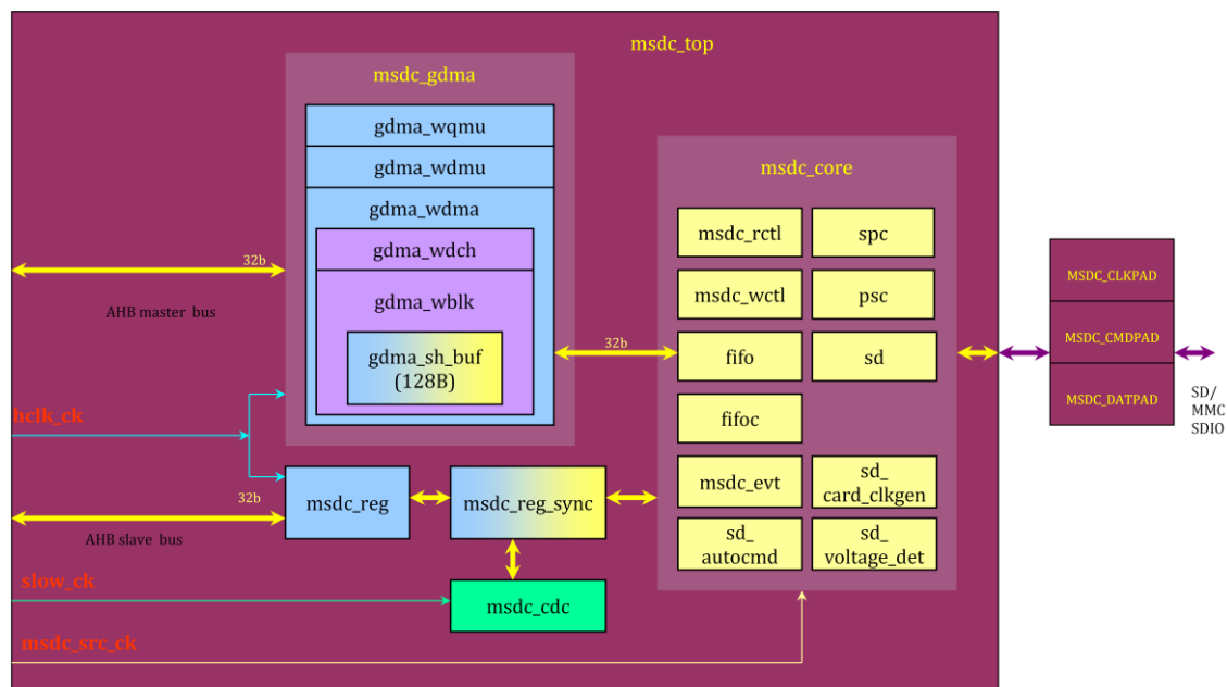
Figure 5-22. MSDC2 controller block diagram
