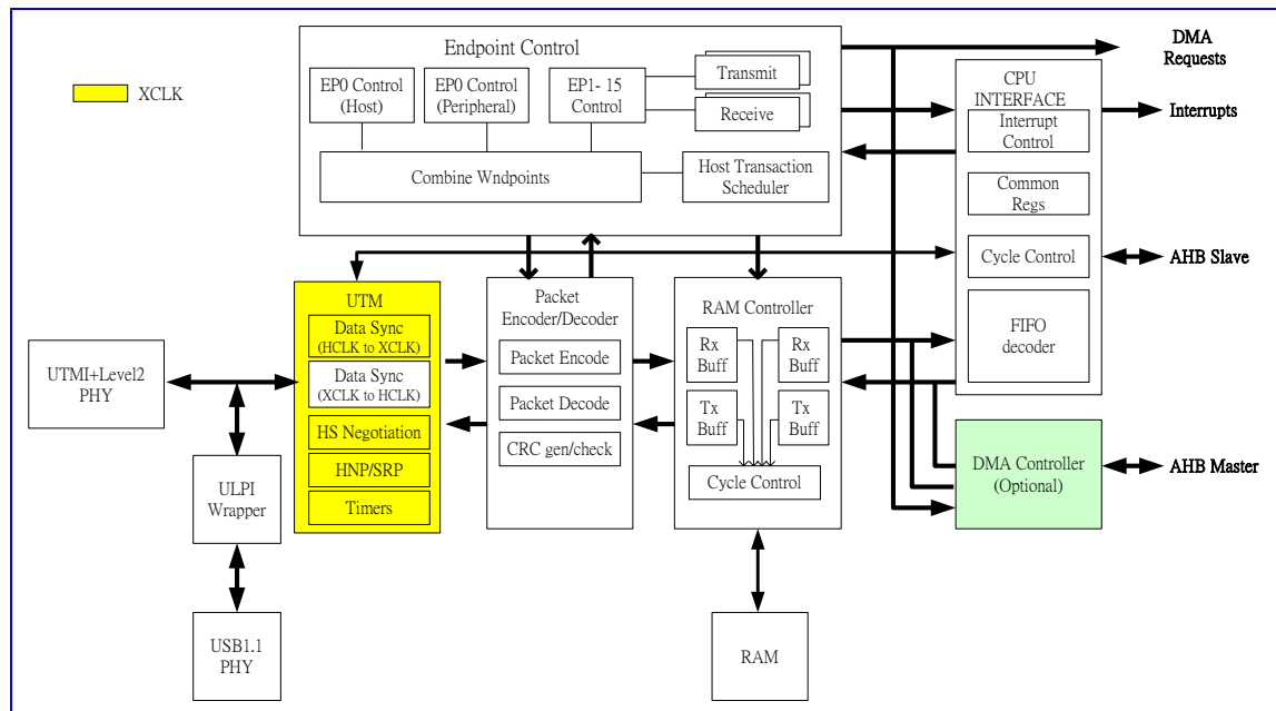
Figure 5-13. USB controller block diagram
