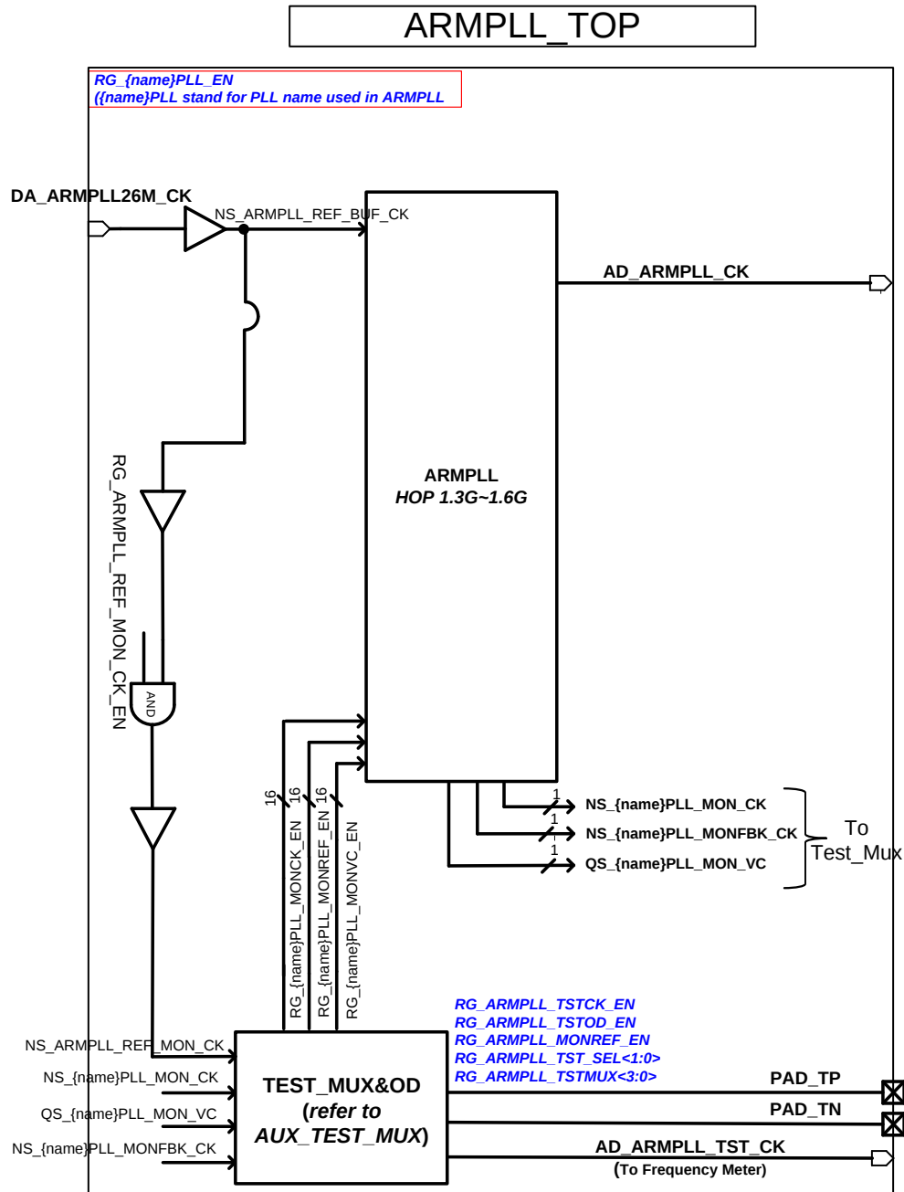
Figure 2-17. Block diagram of ARMPLL
