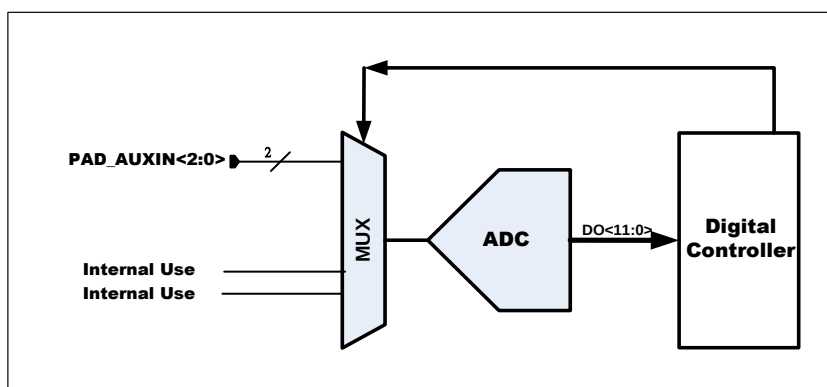
Figure 2-16. Block diagram of AUXADC
