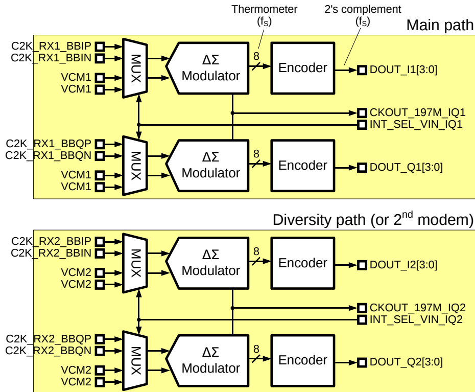
Figure 2-11. Block diagram of C2K_BBRX-ADC
