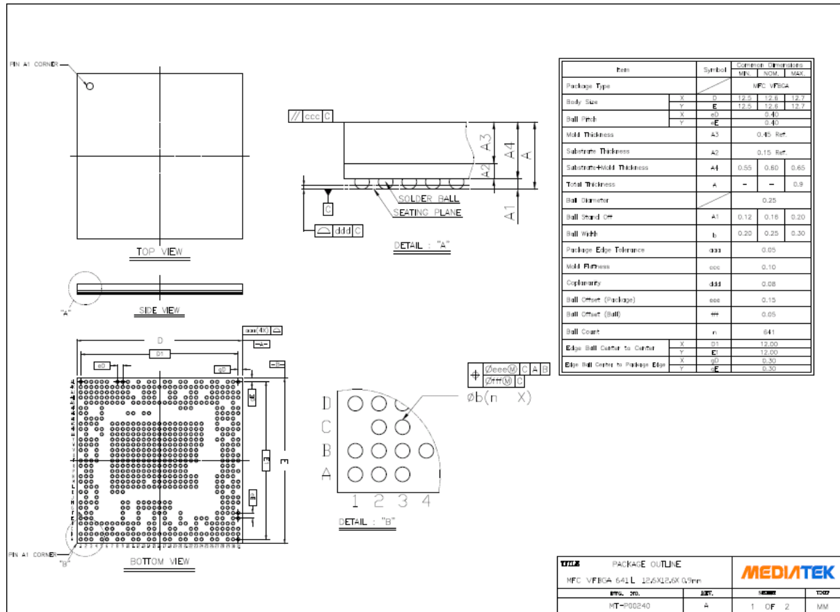
Figure 2-19. Outlines and dimensions of VFBGA 12.6mm*12.6mm, 641 balls, 0.4mm pitch package
