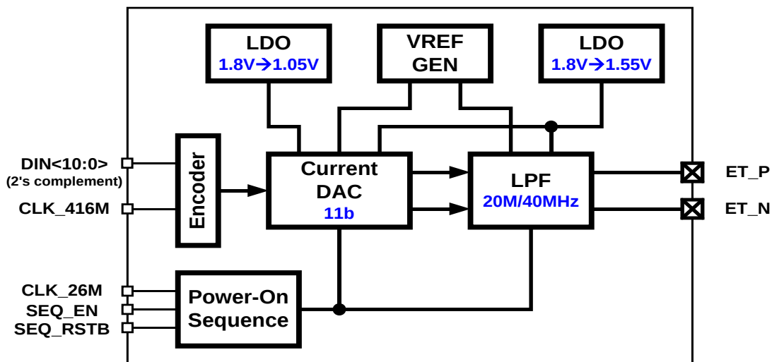
Figure 2-14. Block diagram of ETDAC
