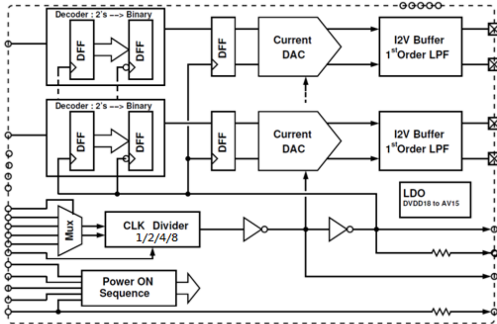
Figure 2-13. Block diagram of C2K_BBTX
