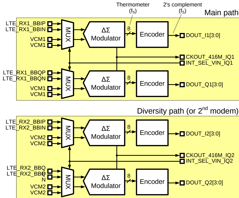
Figure 2-10. Block diagram of LTE_BBRX-ADC
