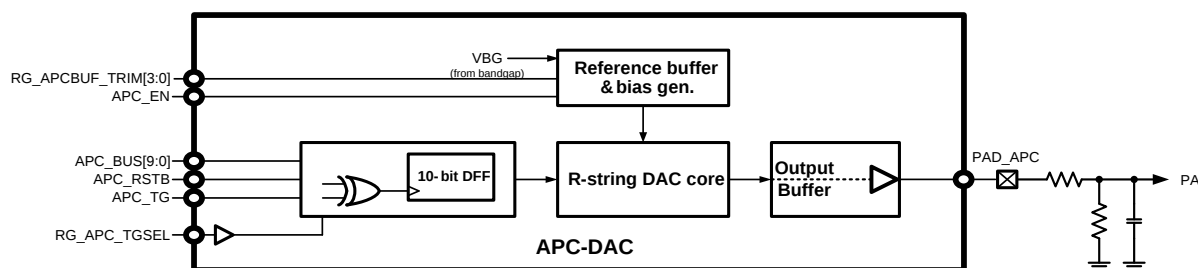
Figure 2-15. Block diagram of APC-DAC (same architecture for two APC-DACs)
