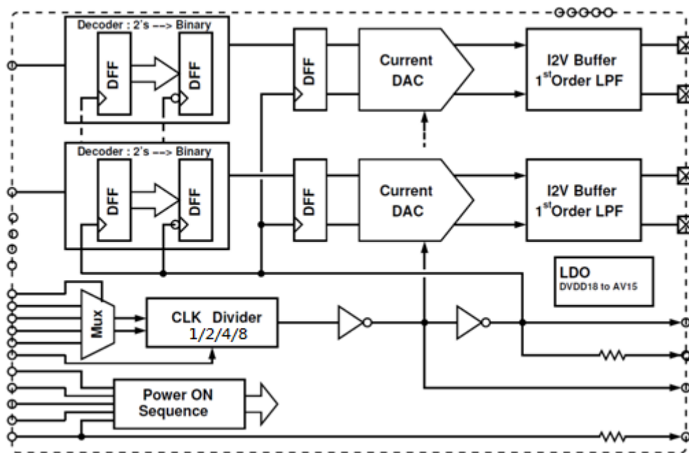
Figure 2-12. Block diagram of LTE_BBTX
