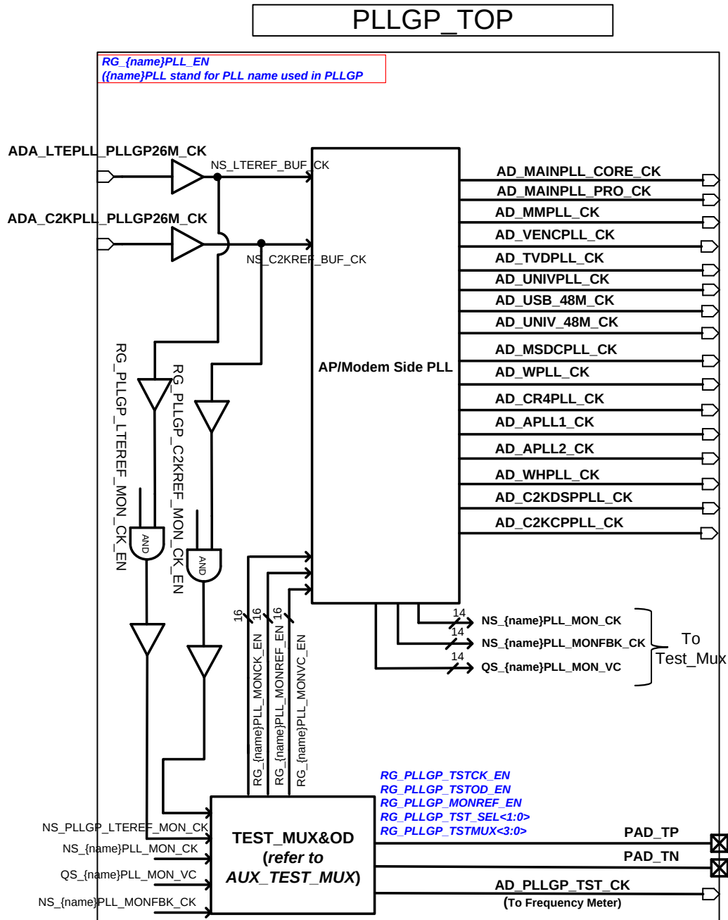
Figure 2-18. Block diagram of PLLGP
