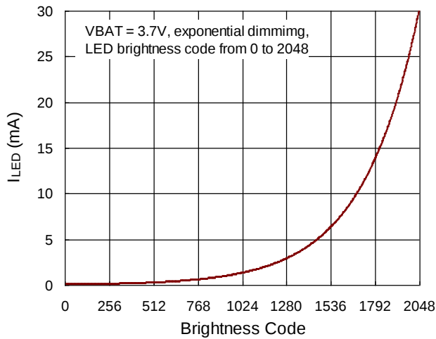
BLED I_{LED} vs. Brightness Code
