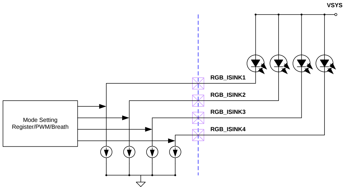
Figure 4-22. RGB LED driver application circuit
