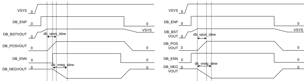
(a) Display Bias delay no constraint
