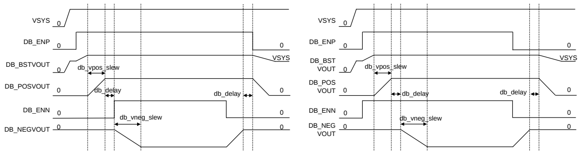
(b) Display Bias delay between DB_POSVOUT and DB_NEGVOUT
