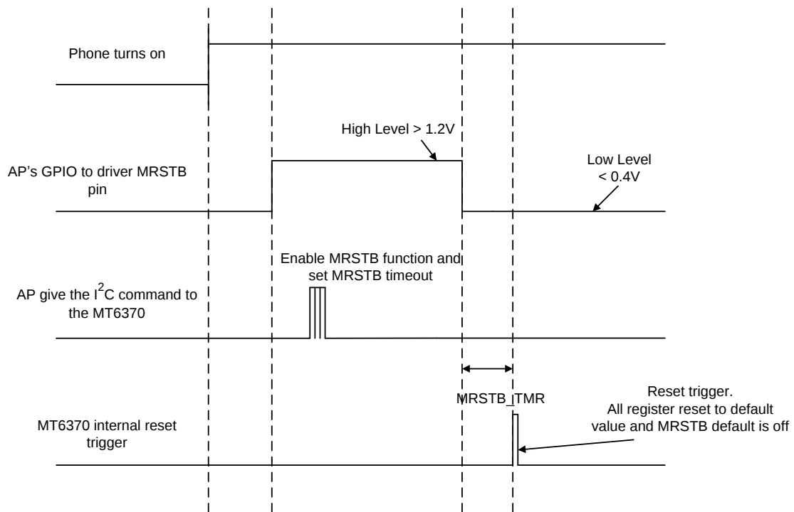
Figure 4-1. MRSTB function
