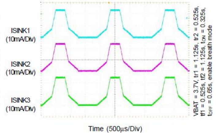
RGB in Breath Mode
