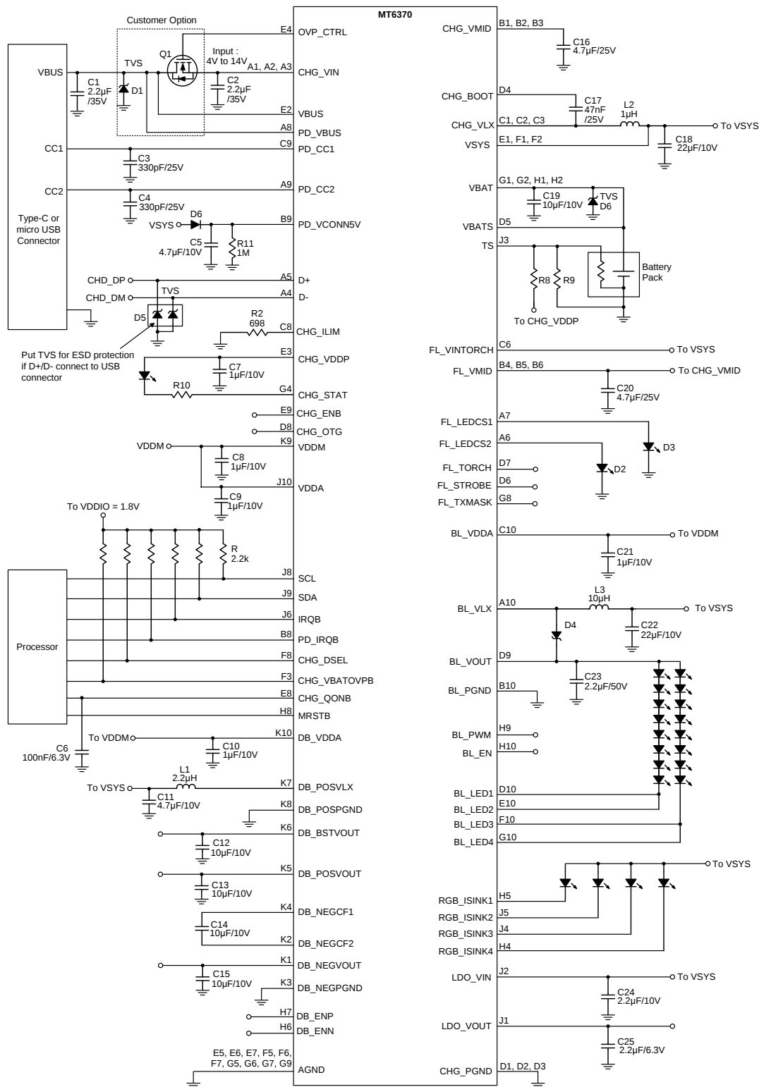
Figure 1-3. With external OVP function
