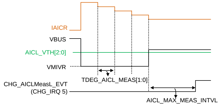
Figure 4-3. Average input current level
