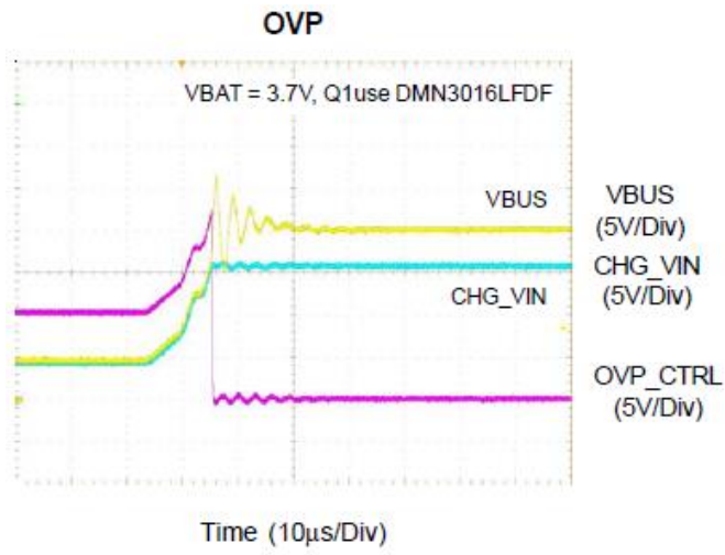
Figure 3-1. Typical operating characteristics
