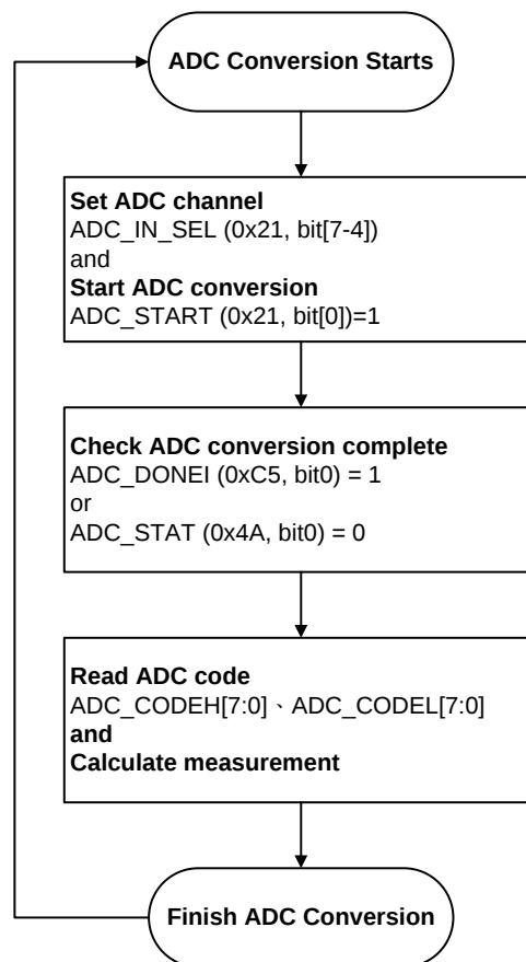
Figure 4-6. ADC conversion operation flow
