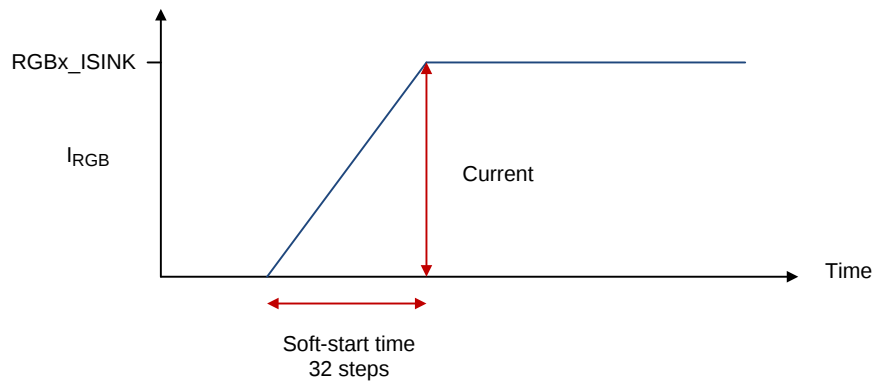
Figure 4-25. RGB register mode operating principle
