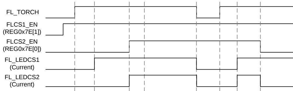
Figure 4-13. FLCS1_EN and FLCS2_EN (FL_TORCH)
