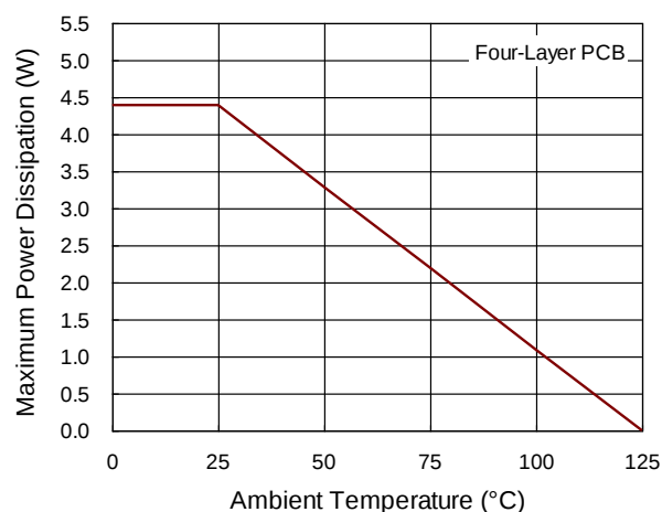
Figure 4-30. Derating curve of maximum power dissipation
