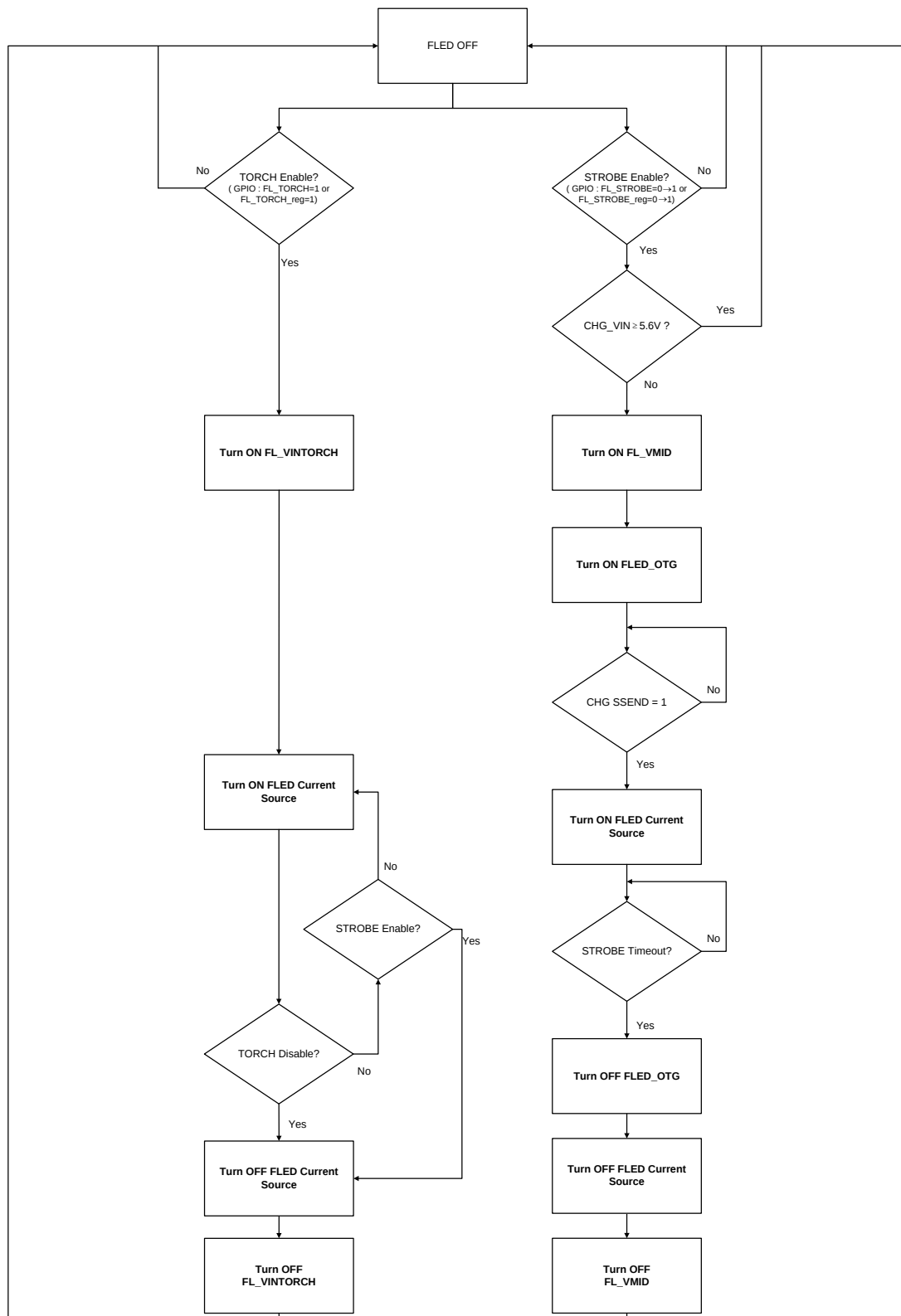
Figure 4-10. FLED flow chart
