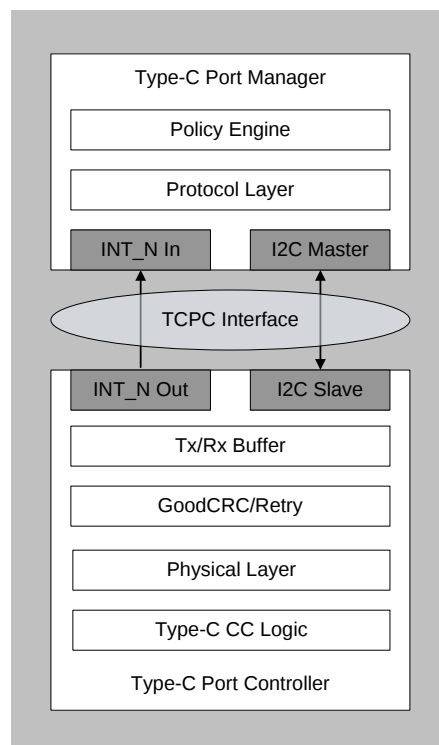
Figure 4-7. Type-C port controller (TCPC) interface
