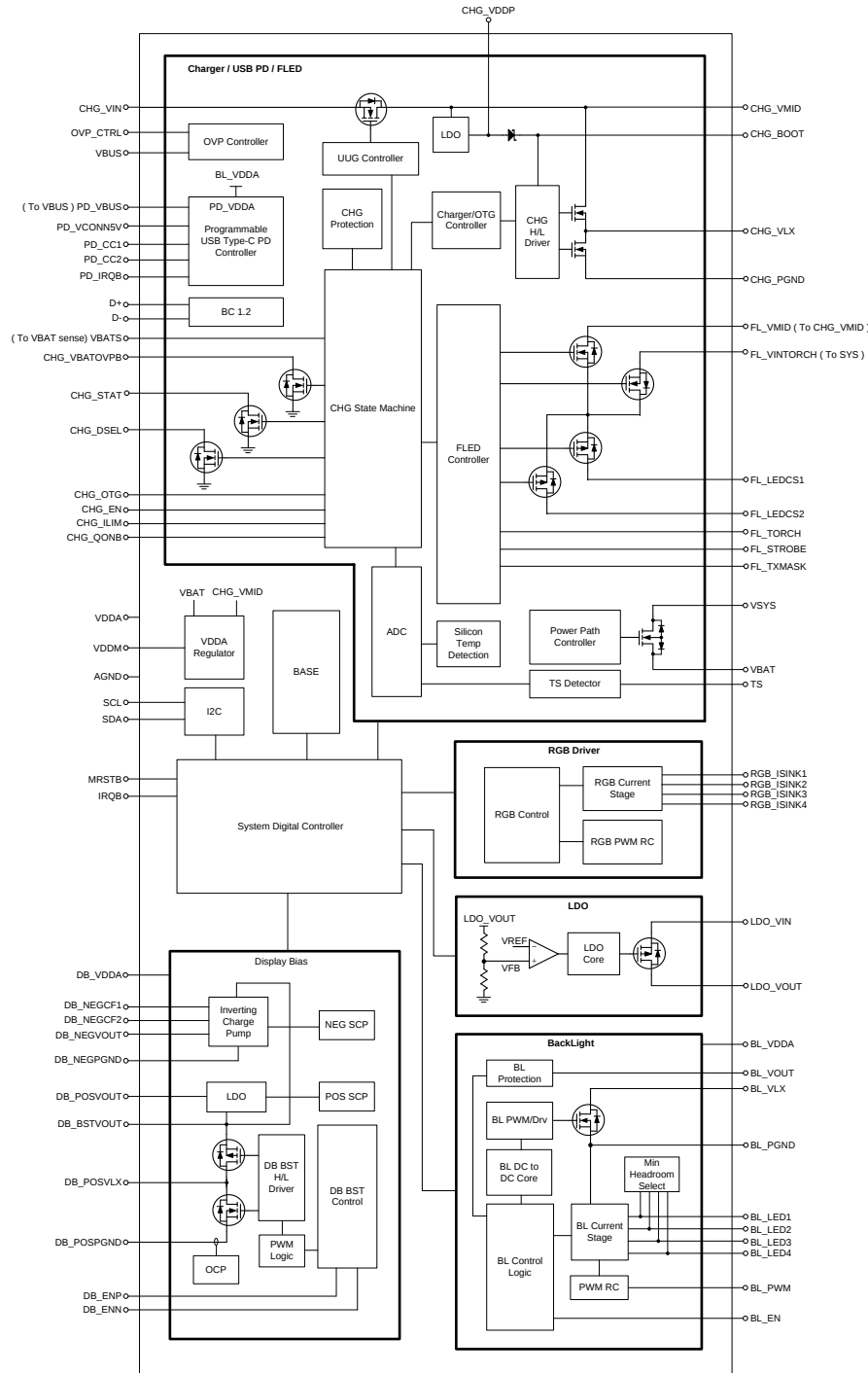
Figure 5-1. MT6370 functional block diagram
