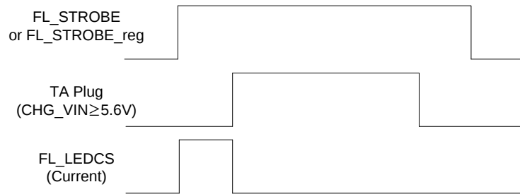
Figure 4-19. Strobe case (CHG_VIN ≥ 5.6V)
