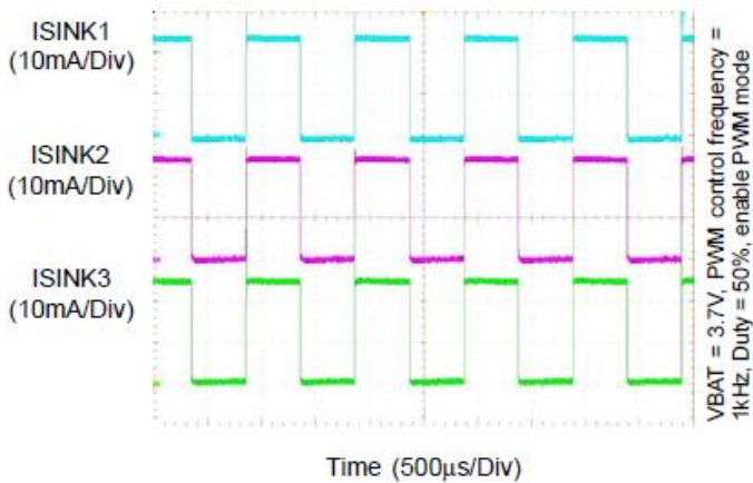
RGB in PWM Mode
