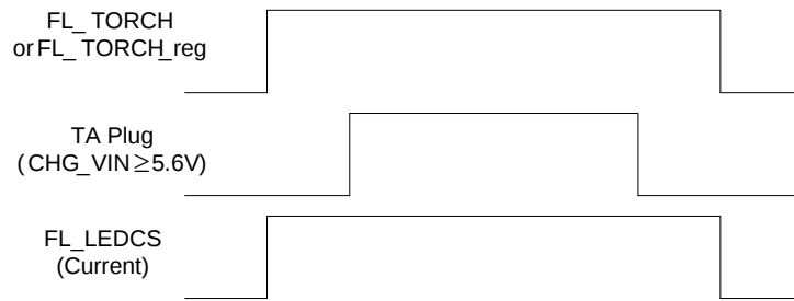
Figure 4-18. Torch case (CHG_VIN ≥ 5.6V)
