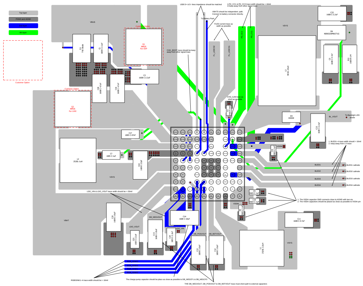
(b) With external OVP function Figure 4-31. PCB layout guide
