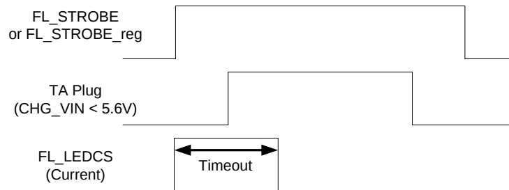
Figure 4-17. Strobe case ( CHG\_VIN < 5.6V )
