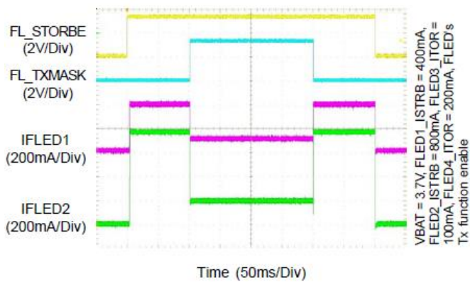
Txmask Behavior
