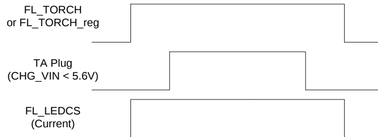
Figure 4-16. Torch case ( CHG\_VIN < 5.6V )
