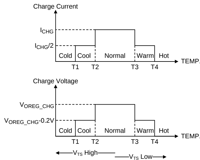
Figure 4-4. JEITA protection
