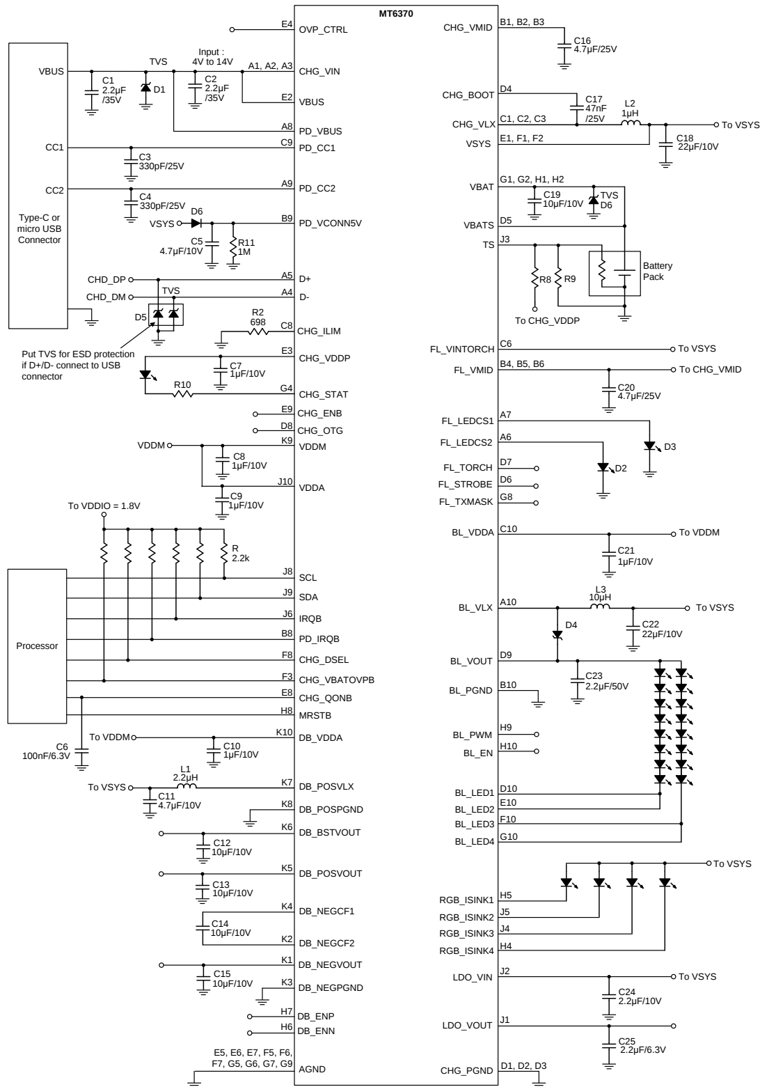
Figure 1-2. Without external OVP function
