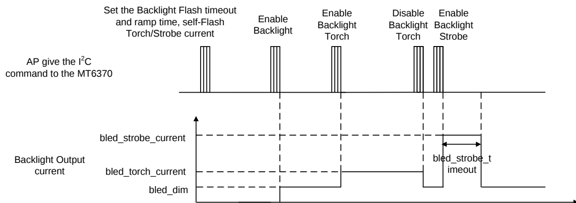
Figure 4-28. Backlight strobe mode case2
