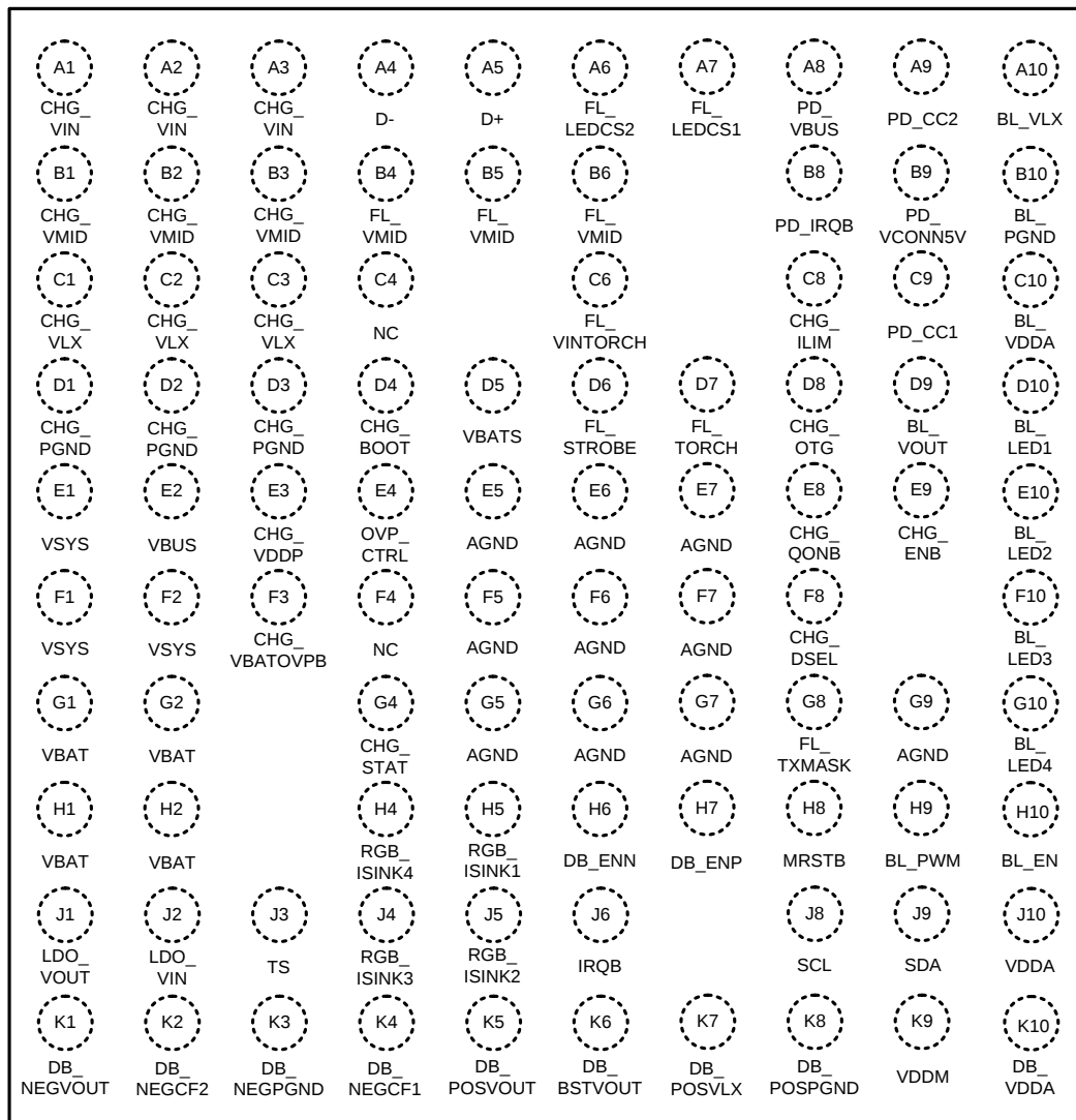
Figure 1-1. MT6370 WL-CSP-93B 4.22x4.32 (BSC) (top view)
