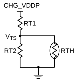
Figure 4-5. Register design for JEITA protection
