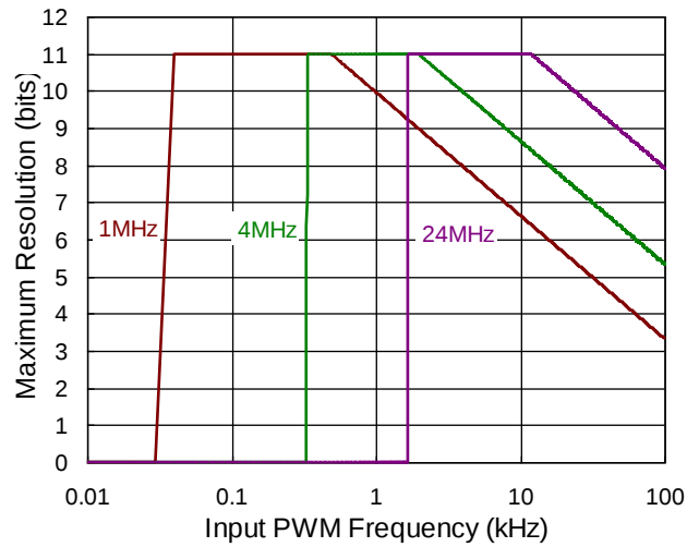
Figure 4-26. PWM sample rate, maximum resolution vs. input PWM frequency
