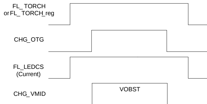
Figure 4-20. Torch case with OTG
