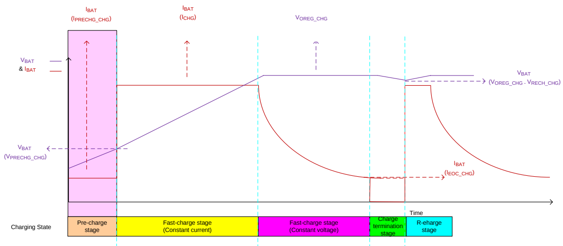
Figure 4-2. Charge profile
