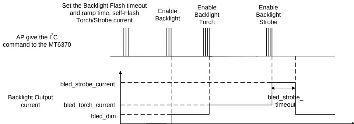
Figure 4-27. Backlight strobe mode case 1
