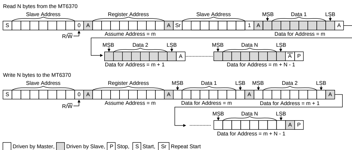
Figure 4-29. I 2 C timing diagrams
