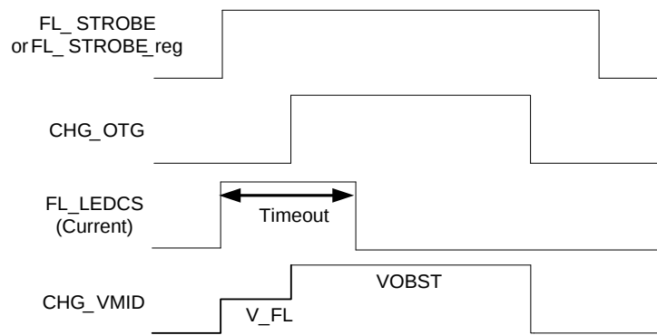
Figure 4-21. Strobe case with OTG
