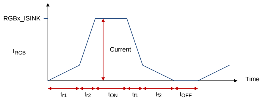
Figure 4-24. RGB breath mode operating principle
