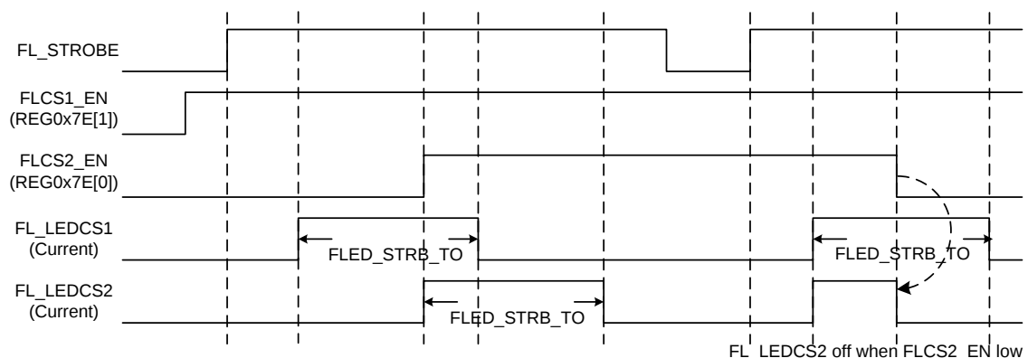
Figure 4-11. FLCS1_EN and FLCS2_EN (FL_STROBE)
