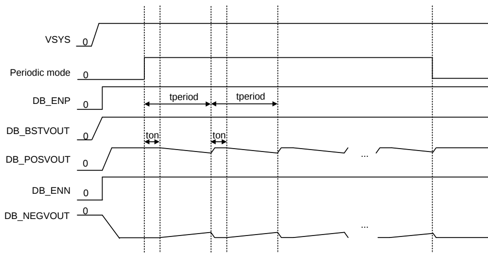
Figure 4-9. Periodic mode control
