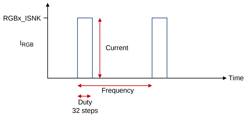
Figure 4-23. RGB PWM mode operating principle
