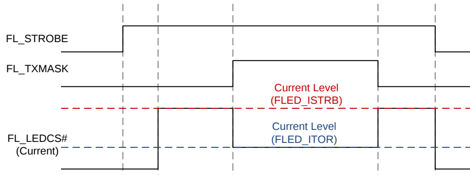
Figure 4-15. FL_TXMASK function
