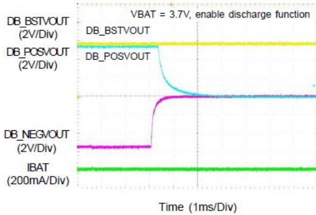
DB Power Off with Delay Function
