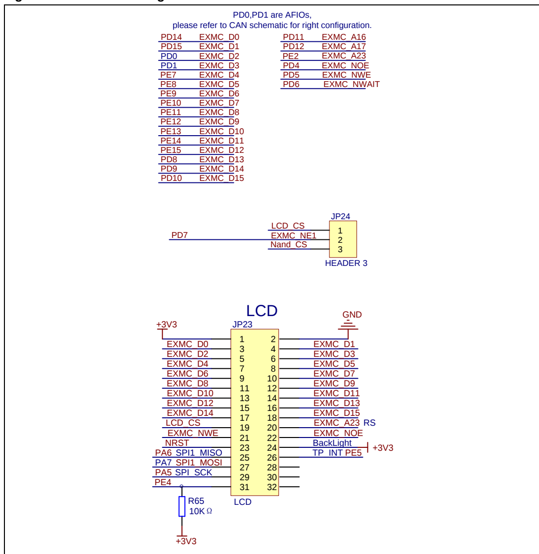
Figure 13. Schematic diagram of EXMC-LCD function
